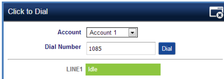
Figure 4: Click-to-Dial
